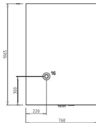
Top view UB 750
